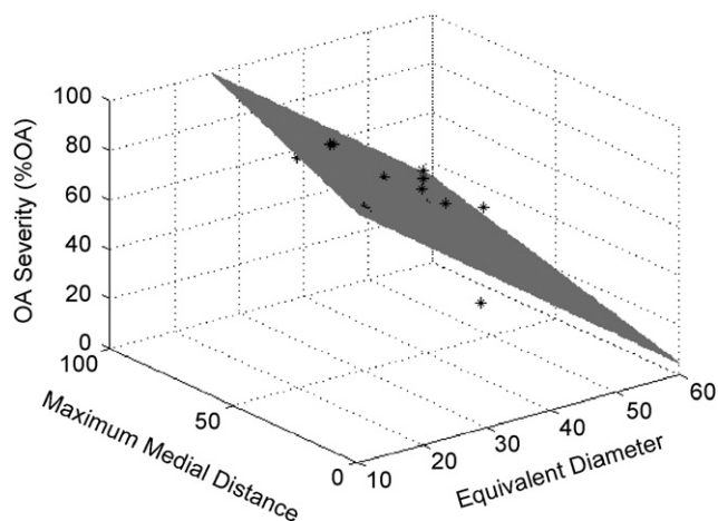
Fig. 6. Three-dimensional scatter diagram and regression surface of the multiple regression analysis model for quantitative estimation of osteoarthritis (OA) severity.
