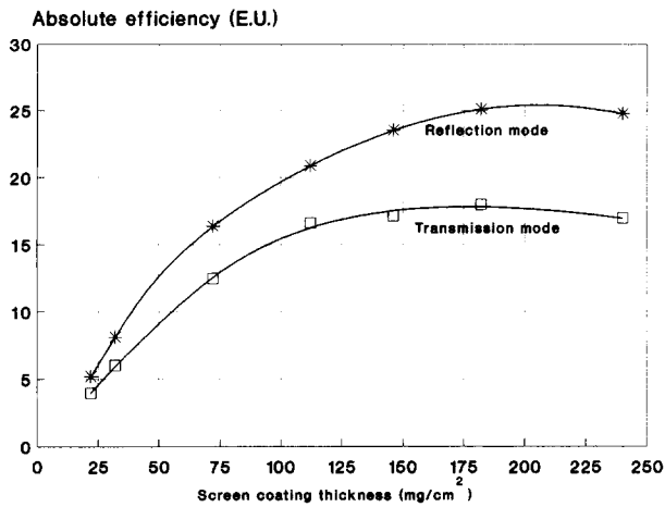
FIG. 3. Variation of x-ray absolute efficiency of \text{Y}_2\text{O}_3:\text{Eu}^{3+} screens with coating thickness in transmission and reflection mode of measurement at 80 kVp. (1 Efficiency Unit, 1 EU = 1 \mu\text{W m}^{-2}/\text{mR s}^{-1} or 3.875 \text{ J/C kg}^{-1} \text{ m}^2 S.I. units.)
