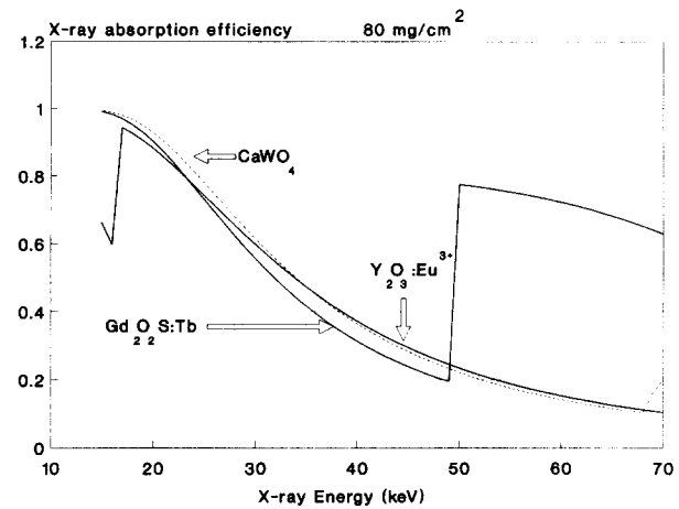
FIG. 4. Variation of absorption efficiency with x-ray energy of \text{Gd}_2\text{O}_2\text{S:Tb} , \text{CaWO}_4 , and \text{Y}_2\text{O}_3:\text{Eu}^{3+} 80 \text{mg/cm}^2 screens.
