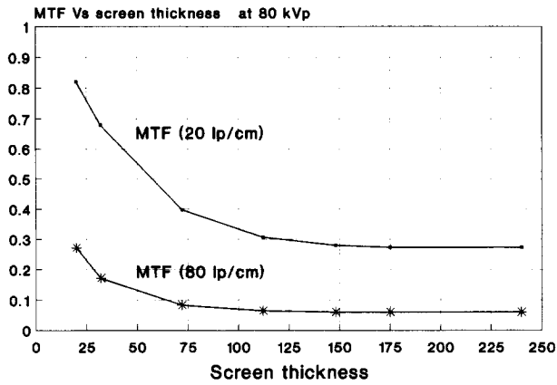
FIG. 9. Variation of Y_2O_3:Eu^{3+} MTFs with screen thickness at 80 lp/cm and at 20 lp/cm.
