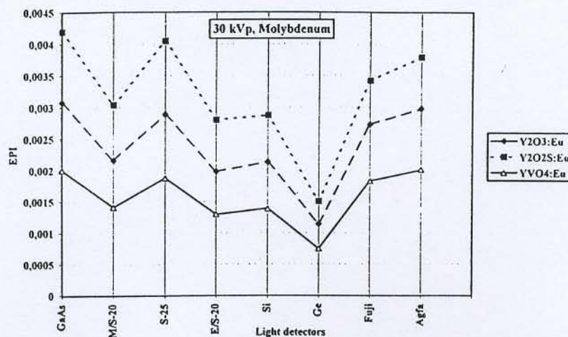
Fig. 5. Effective performance index (EPI) of Y_2O_2S:Eu , Y_2O_3:Eu and YVO_4:Eu phosphors in combinations with various optical detectors, determined at 30 kVp using molybdenum target X-rays.
