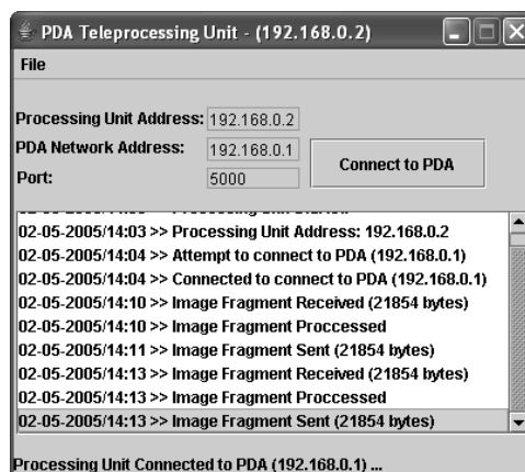
Figure 3. Client-side application running on a PU
