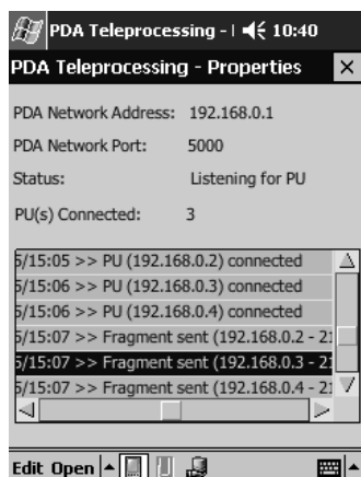
Figure 2. Server-side application running on a PDA
