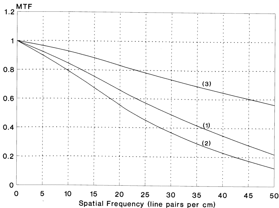
Figure 7. The MTF curve of the video acquisition system (1) and the measured (2) and corrected (3) MTF curves of a 30 \text{ mg cm}^{-2} \text{La}_2\text{O}_2\text{S:Tb} phosphor screen.
