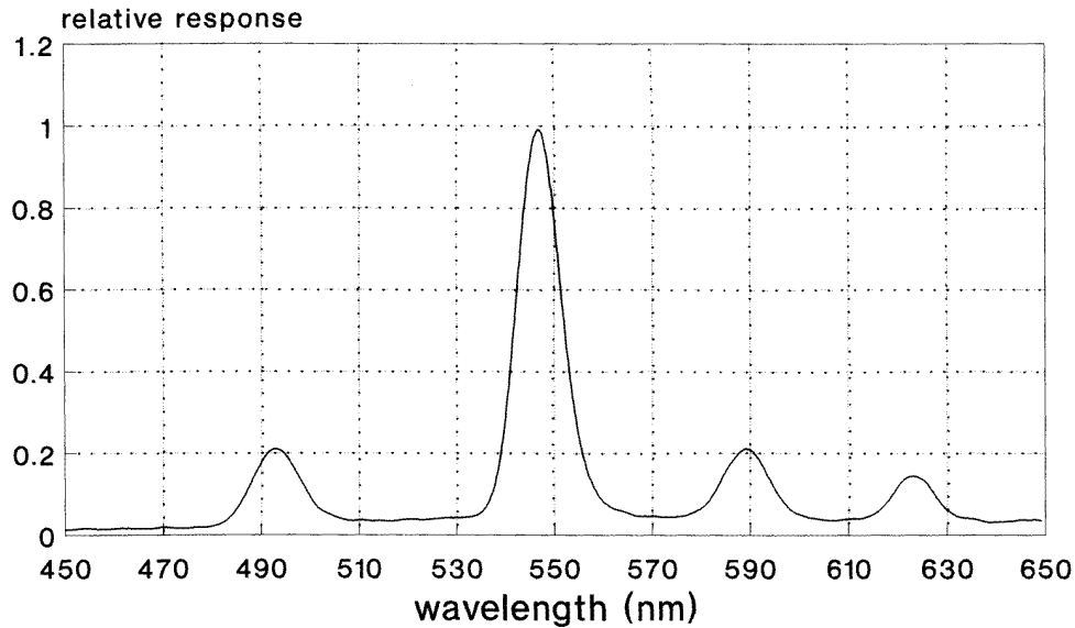
Figure 1. The spectral response of the \text{La}_2\text{O}_2\text{S:Tb} screen.
