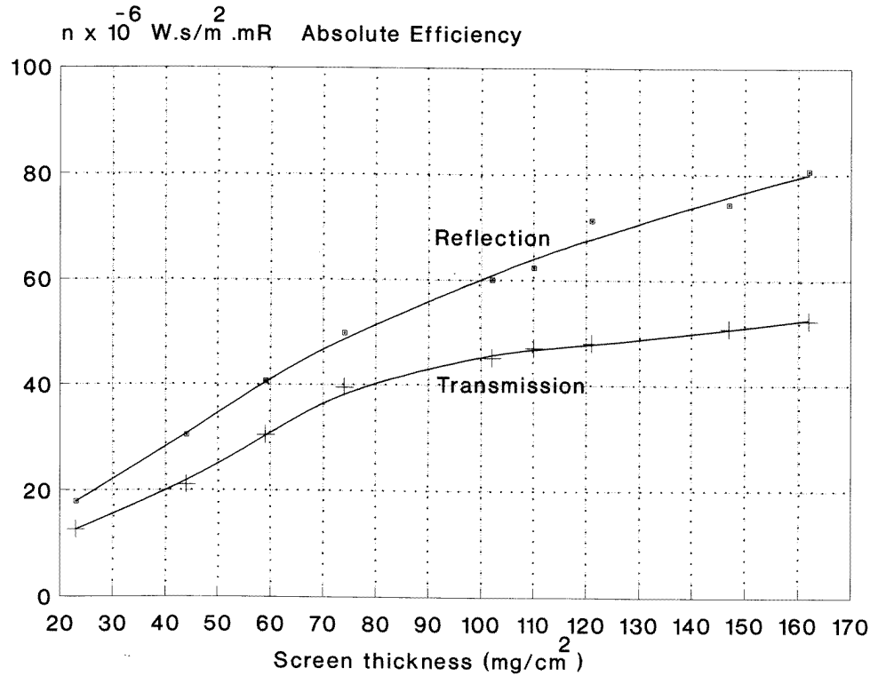
Figure 4. Absolute efficiency of La 2 O 2 S:Tb screens versus screen's coating thickness for both reflection and transmission mode, for 80 kVp x-ray tube voltage. Solid lines, theoretical results; points, experimental data.
