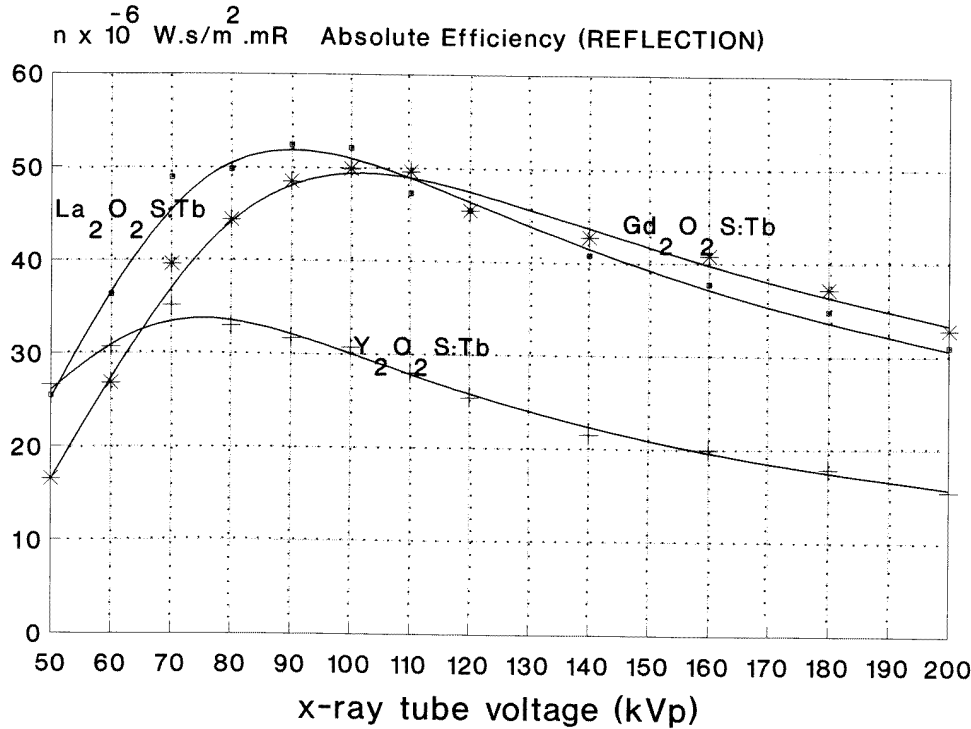
Figure 5. The variation of absolute efficiency measured in reflection mode for Y_2O_2S:Tb , La_2O_2S:Tb and Gd_2O_2S:Tb screens of approximately the same coating thickness ( 70 \text{ mg cm}^{-2} ). Solid lines, theoretical results; points, experimental data.
