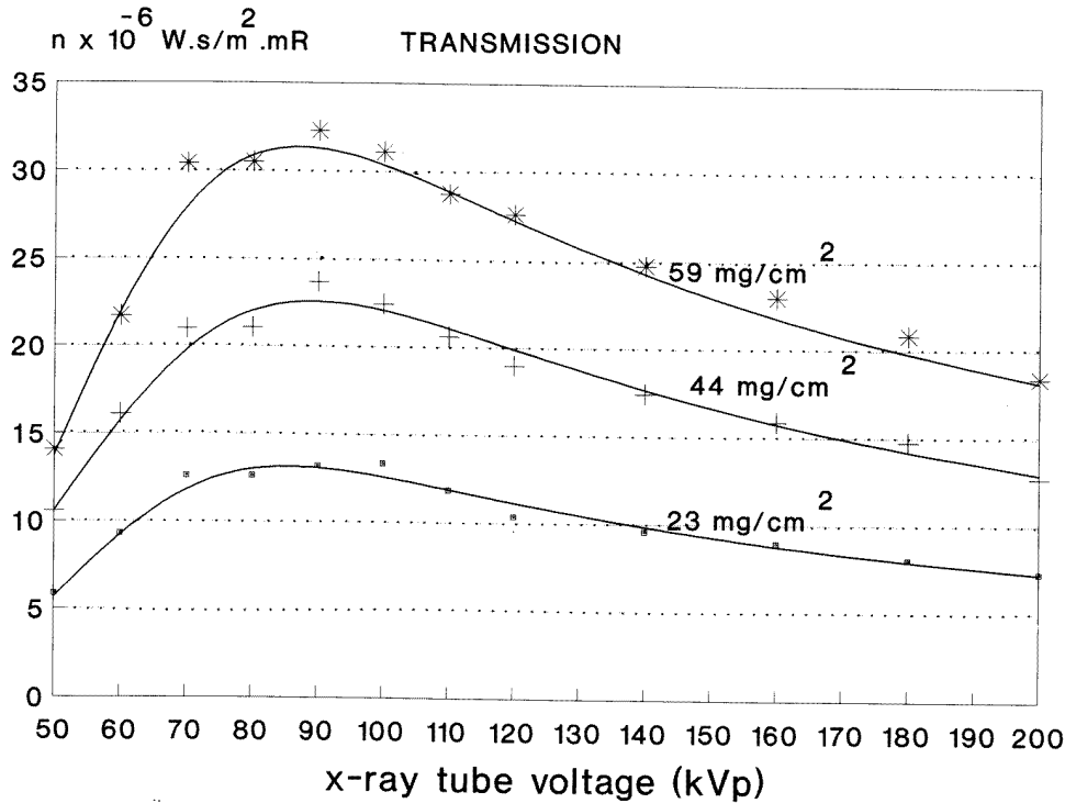
Figure 2. Absolute efficiency in transmission mode versus x-ray tube voltage for three La 2 O 2 S:Tb screens of 23, 44, and 59 mg cm -2 coating thickness. Solid lines, theoretical results; points, experimental data.
