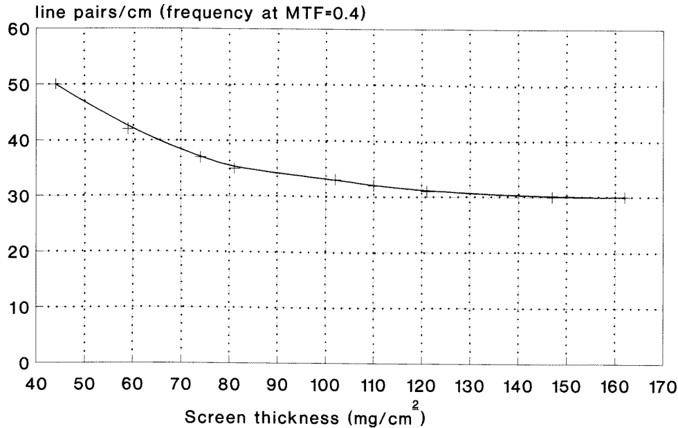
Figure 8. Calculated values of resolution (frequency at MTF = 0.4) against screen coating thickness for La 2 O 2 S:Tb screens.
