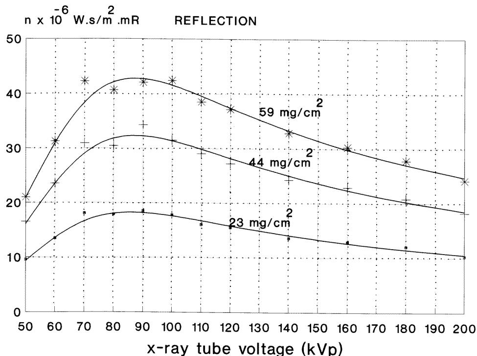
Figure 3. Absolute efficiency in reflection mode versus x-ray tube voltage for three \text{La}_2\text{O}_2\text{S:Tb} screens of 23, 44, and 59 \text{mg cm}^{-2} coating thickness. Solid lines, theoretical results; points, experimental data.
