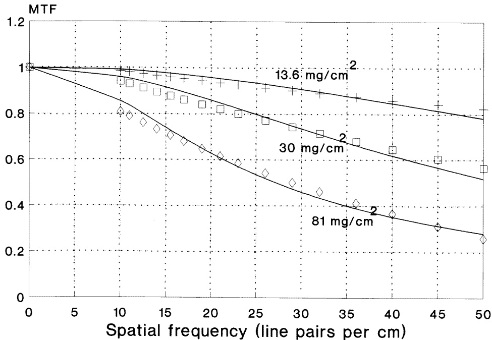
Figure 6. MTF curves for three La 2 O 2 S:Tb screens of 13.6, 30, and 81 mg cm -2 coating thickness. Solid lines, calculated MTF values; points, experimental data.
