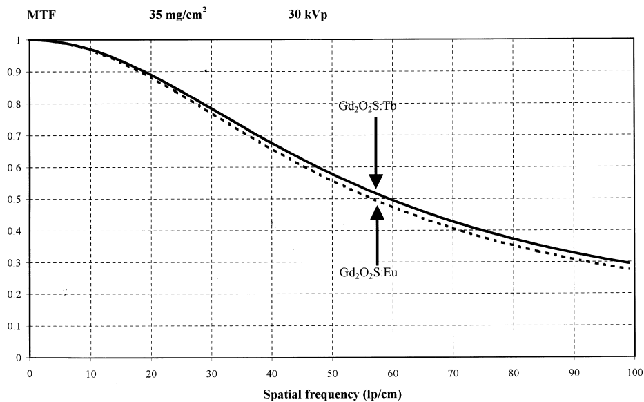
Fig. 4. Comparison of the modulation transfer functions of Gd 2 O 2 S:Tb and Gd 2 O 2 S:Eu scintillators determined in transmission mode.
