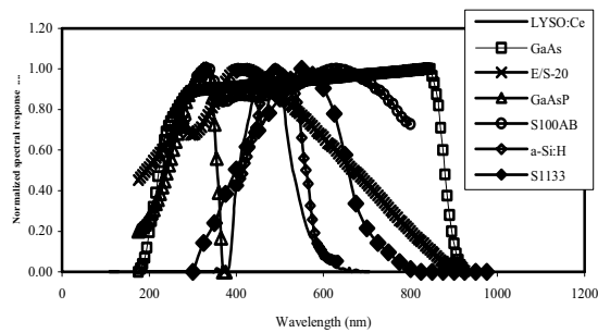
Figure 3. Normalized spectral response of LYSO: Ce compared to the spectral sensitivities of GaAs, ES-20, GaAsP, CCD S100AB, a-Si:H 108H and S1133 photodetectors.
