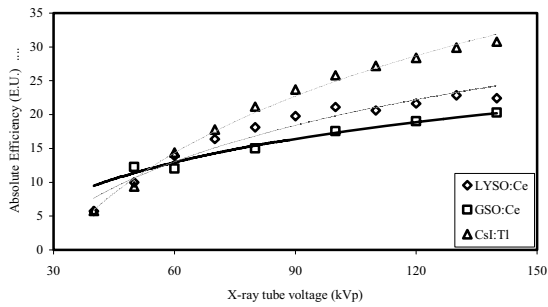
Figure 1 Variation of absolute luminescence efficiency (AE) of LYSO: Ce, GSO: Ce and CsI: Tl crystals for Radiographic X-ray tube voltages, between 40 and 140 kV. AE units: \mu\text{W} \cdot \text{s} / \text{mR} \cdot \text{m}^2 . Points: measured data, line: fitted curve.
