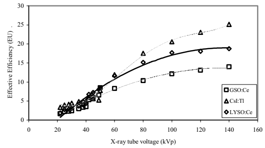
Figure 5. Effective efficiency of LYSO: Ce, GSO: Ce and CsI: Tl crystals using aSi:H-108H amorphous silicone photodiode with intrinsic layer thickness 800nm
