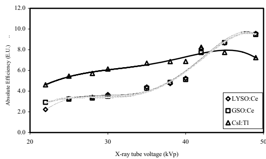
Figure 2. Variation of absolute luminescence efficiency (AE) of LYSO: Ce, GSO: Ce and CsI: Tl crystals for Mammography x-ray tube voltages, between 22 and 49 kV. AE units: \mu\text{W} \cdot \text{s} / \text{mR} \cdot \text{m}^2 . Points: measured data, line: fitted curve.
