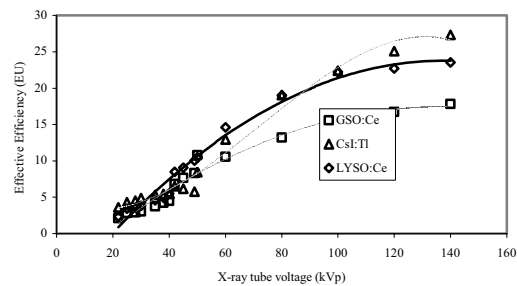
Figure 8. Effective efficiency of LYSO: Ce, GSO: Ce and CsI: Tl crystals using CCD S100AB SiTe photodetector
