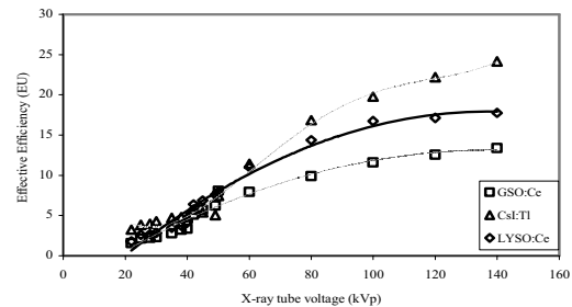
Figure 7. Effective efficiency of LYSO: Ce, GSO: Ce and CsI: Tl crystals using GaAsP Hamamatsu photocathode
