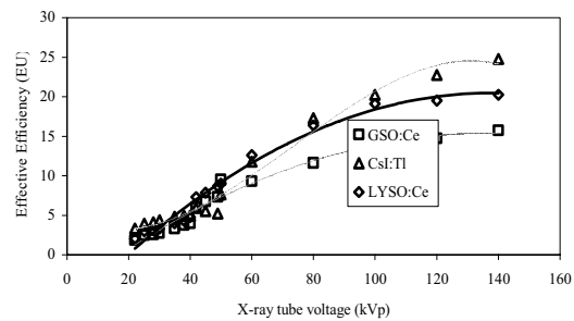
Figure 6. Effective efficiency of LYSO: Ce, GSO: Ce and CsI: Tl crystals using Si/S1133 crystalline silicone Hamamatsu photodiode.
