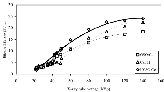
Figure 4. Effective efficiency of LYSO: Ce, GSO: Ce and CsI: Tl crystals using S-20 EMI photocathode
